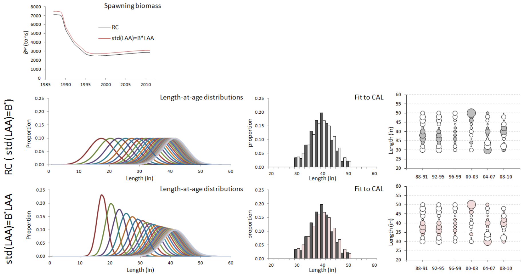
Figure 14: Trajectories of spawning biomass, length-at-age distribution, and fits to the CAL data for the RC and the sensitivity in which the standard deviation of the length-at-age distribution is length dependent ( S13 ).
