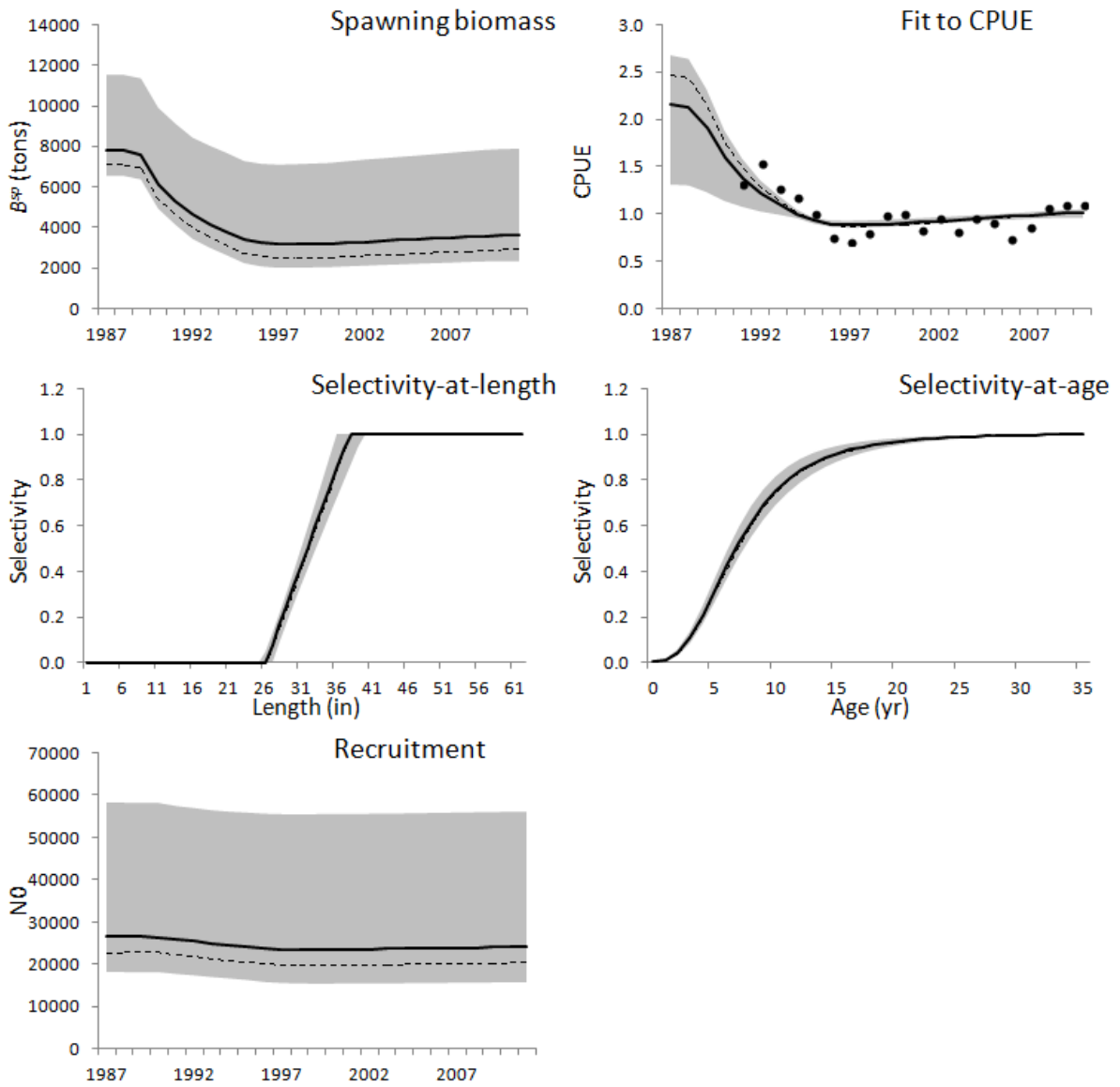
Figure 19a: Median and lower and upper 5%iles trajectory projections for the Bayesian RC. The dashed curves show the MLEs, and the solid curves reflect the posterior medians, while the shading shows the 90% posterior probability envelopes.
