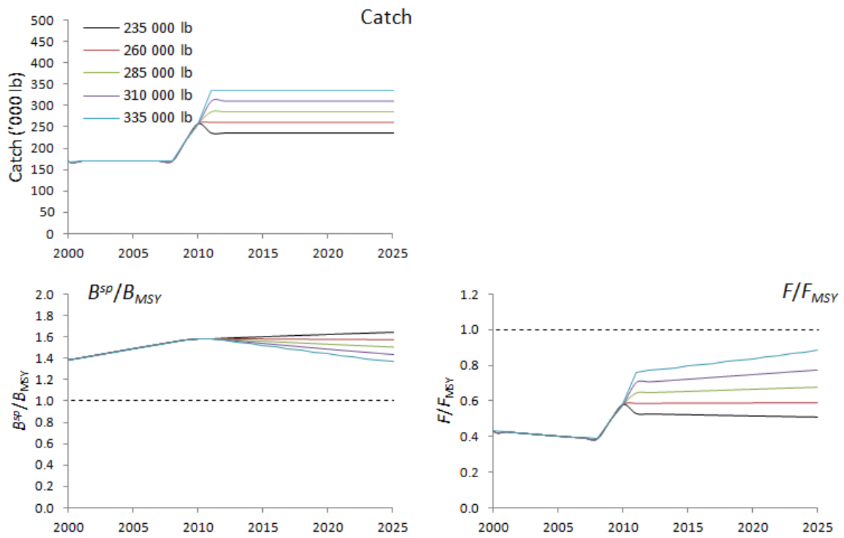
Figure 18: Catch, spawning biomass (relative to B_{MSY} ) and fishing mortality (relative to F_{MSY} ) trajectories under a series of constant catch projections for the RC.
