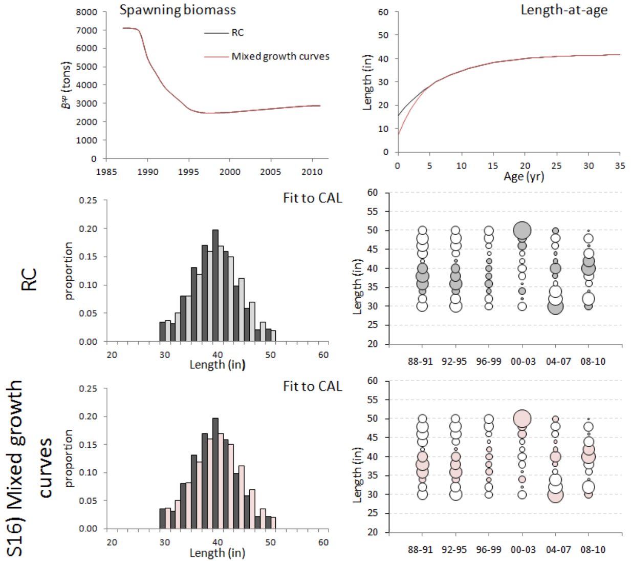
Figure Add.2: Spawning biomass trajectories, growth curves and fits to the CAL data (averaged over all the years for which data are available together with bubble plots of residuals) for the RC and the sensitivity with mixed growth curves (S16).
