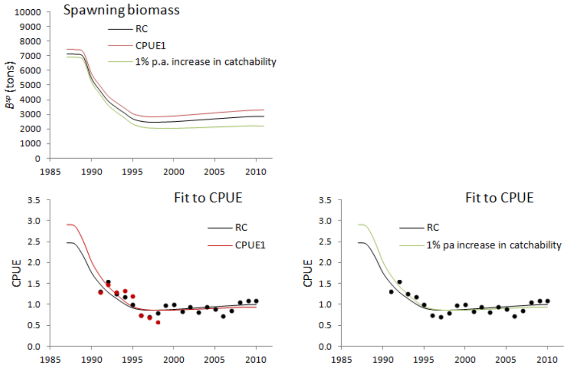
Figure 5: Spawning biomass trajectories, with fits to the CPUE data for the RC and two sensitivities involving CPUE. For CPUE1, the 1991-1998 CPUE data points have been replaced by the Vaughan et al. (S4a) (2001) series, renormalized to the average of the RC series over the same period. The new CPUE data points are shown as red dots in the left-hand plot. The 1% p.a. increase in catchability run corresponds to S4b.
