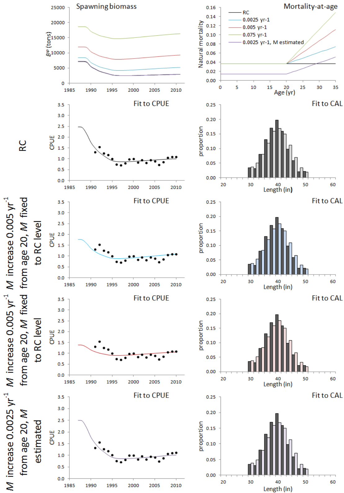
Figure 4: Spawning biomass trajectories for different specifications for natural mortality-at-age showing fits to the CPUE and CAL data (averaged over all the years for which data are available) for the RC and four sensitivities with increasing natural mortality for older ages ( M increases from the RC level by 0.0025 \text{ yr}^{-1} for S3a , 0.005 \text{ yr}^{-1} for S3b , and 0.0075 \text{ yr}^{-1} for S3c ; and for S3d , M increases from an estimated level by 0.0025 \text{ yr}^{-1} ).
