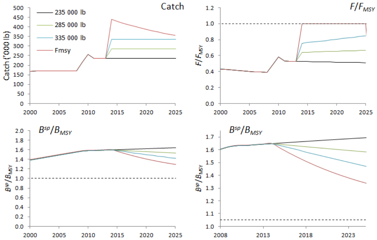
Figure Add.6: MLE catch, spawning biomass (relative to B_{MSY} ) and fishing mortality (relative to F_{MSY} ) trajectories under a series of constant catch and F_{MSY} projections for the deterministic RC.
