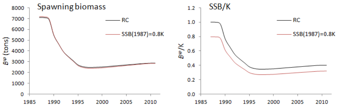
Figure 12: Spawning biomass trajectories in absolute terms and relative to pre-exploitation level for the RC and the sensitivity which fixes the starting 1987 spawning biomass at 0.8 of K ( S11 ).
