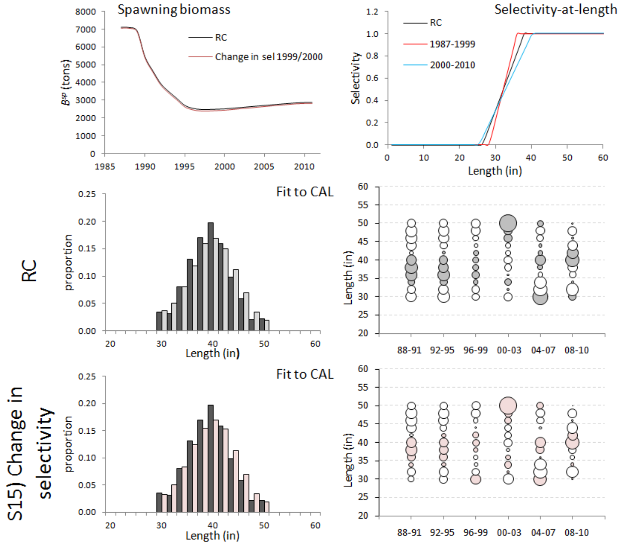
Figure Add.1: Spawning biomass trajectories, selectivities-at-length and fits to the CAL data (averaged over all the years for which data are available together with bubble plots of residuals) for the RC and the sensitivity which allows for a change in the commercial selectivity between 1999 and 2000 (S15).
