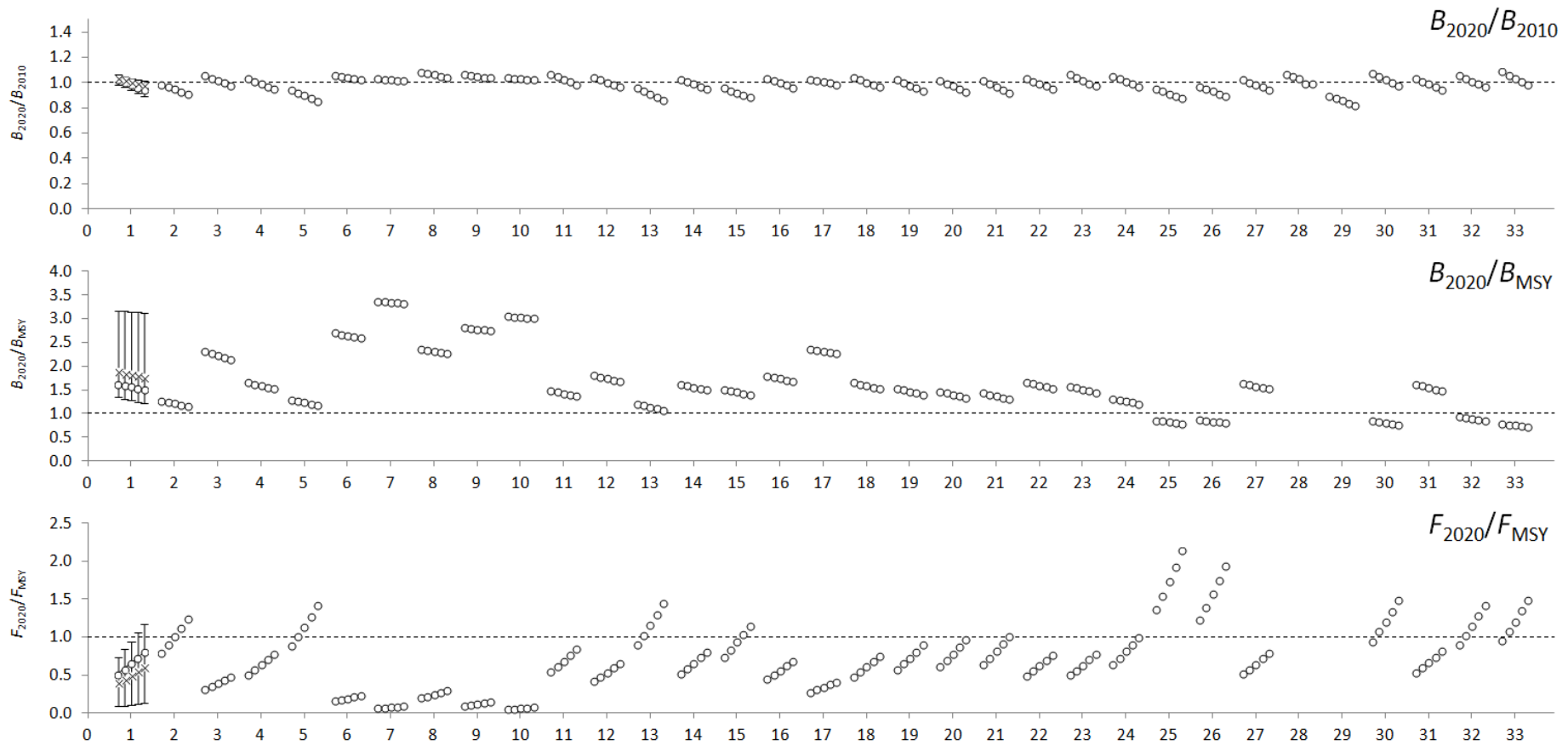
Figure 20: Projections results for the RC and the sensitivities under various future constant catches (235, 260, 285, 310 and 335 thousand lb from left to right respectively). Similar results are also shown for the dynamic production models, for which F refers to the C/B ratio. For the RC, the MLE and posterior median (crosses) with 90% PI as error bars are shown. The runs are shown in the following order:
