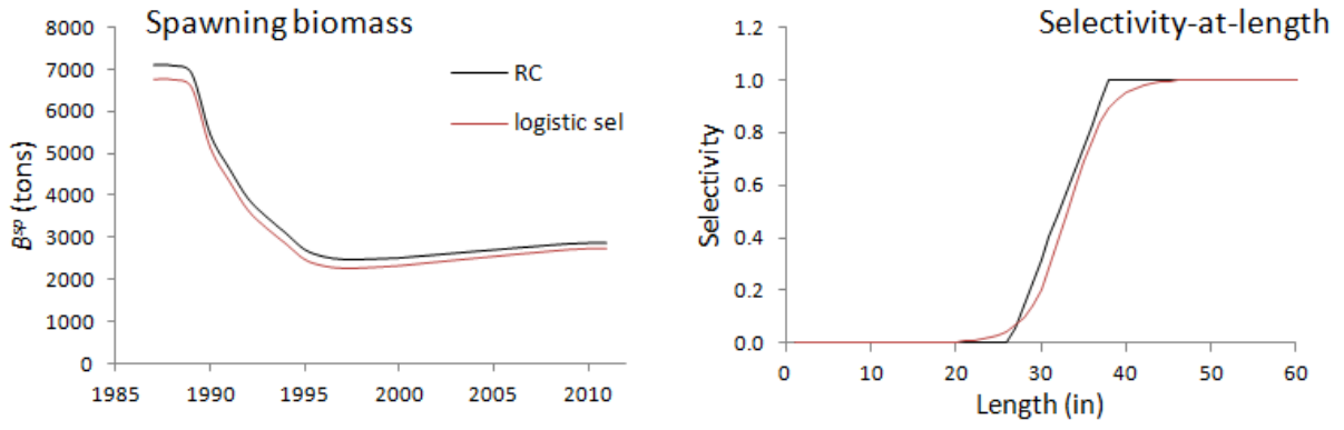
Figure 8: Spawning biomass trajectories and selectivity-at-length for the RC and a sensitivity with an estimated logistic selectivity-at-length function ( S6b ).
