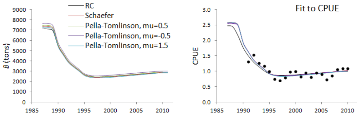
Figure 17: Trajectories of spawning biomass and fit to the CPUE data for the RC, and for the Schaefer and Pella-Tomlinson production models.
