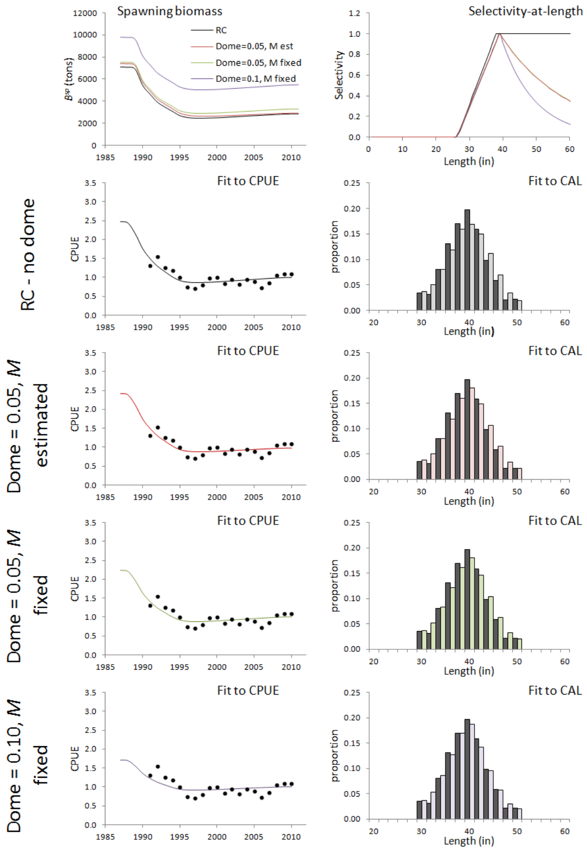
Figure 7: Spawning biomass trajectories, selectivity-at-length and fits to the CPUE and CAL data (averaged over all the years for which data are available) for the RC and three sensitivities with fixed rates of decreasing selectivity (“dome”) at larger lengths (S6a).
