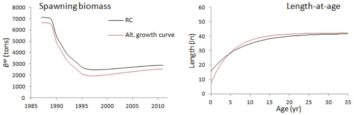
Figure 11: Spawning biomass trajectories and length-at-age for the RC and the sensitivity using an alternative growth curve ( S10 ).
