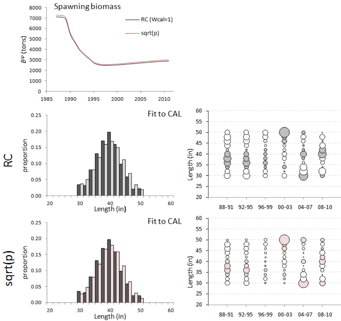
Figure 10: Spawning biomass trajectories and fits to the CAL data (averaged over all the years for which data are available together with bubble plots of residuals) for the RC and the sensitivity using a surrogate of the multinomial for the CAL component of -\ln L(\text{sqrt}(p)) (S9).
