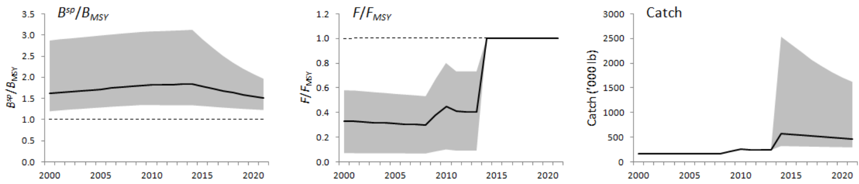
Figure Add.7: Spawning biomass (relative to B_{MSY} ), fishing mortality (relative to F_{MSY} ) and catches median and lower and upper 5%iles Bayesian trajectory projections under constant F_{MSY} projections commencing in 2014 for the Bayesian RC. The solid curves reflect the posterior medians, while the shading shows the 90% posterior probability envelopes.
