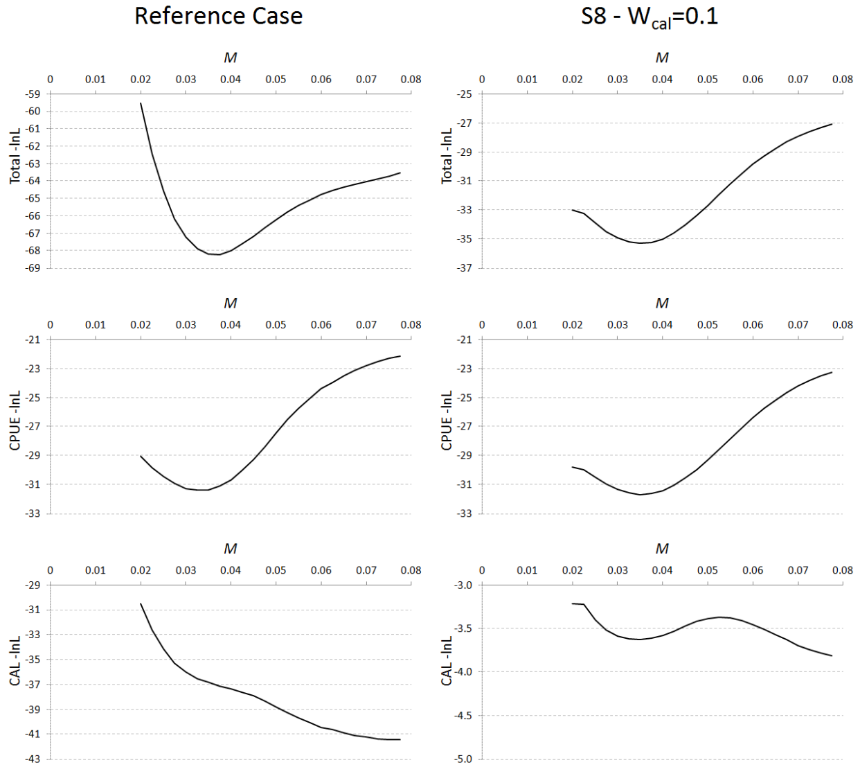
Figure Add.5: Negative log-likelihood profiles for M for the RC and for sensitivity S8c in which the CAL data are downweighted by a multiplicative factor of 0.1.
