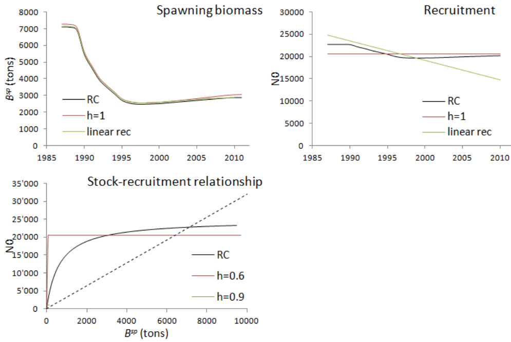
Figure 15: Trajectories of spawning biomass and recruitment for the RC and two alternative stock-structure ( S14a : h=1 ; S14b : linear decrease in recruitment).
