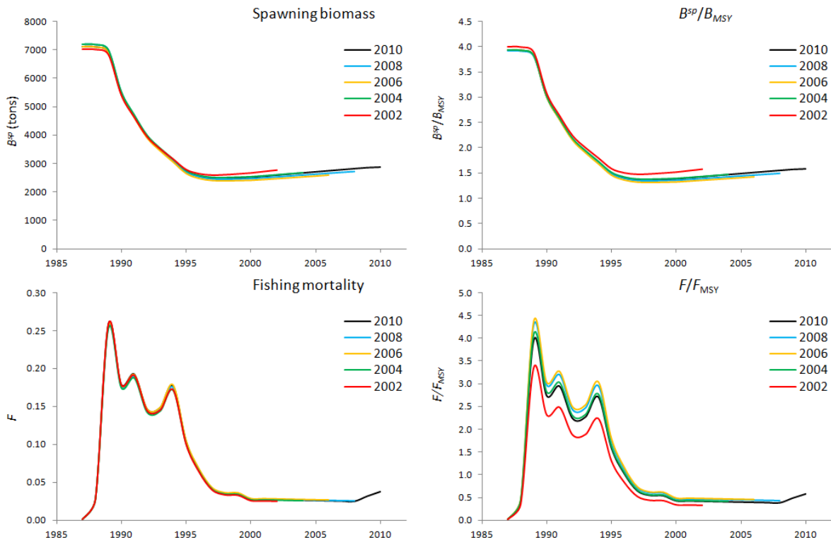
Figure 16: Retrospective results for the RC.
