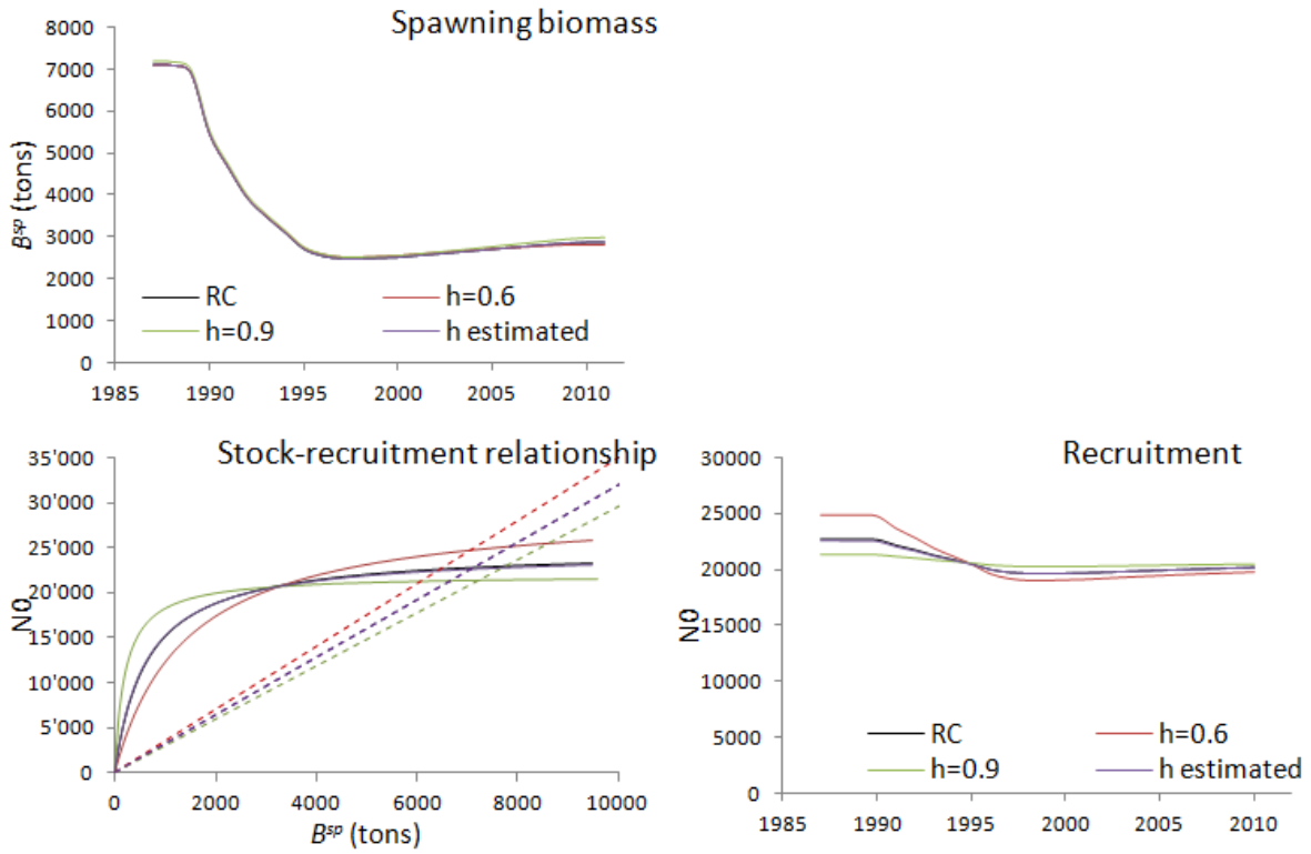
Figure 2: Trajectories of spawning biomass and recruitment, as well as the stock-recruitment relationship for the RC ( h=0.75 ), two sensitivities with different fixed values for the steepness parameter ( S1a : h=0.6 and S1b : h=0.9 ) and a sensitivity in which a prior for h is provided and h is estimated ( S1c : h=0.758 ). The replacement lines are shown as dotted line in the plot of the stock-recruitment relationships.
