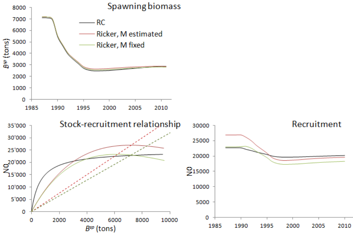
Figure 13: Trajectories of spawning biomass and recruitment, as well as the stock-recruitment relationship for the RC (Beverton-Holt, h=0.75 ) and the two sensitivities using a Ricker stock-recruitment curve with h estimated ( S12a : M is estimated, S12b : M is fixed to the RC level). The replacement lines are shown as dotted lines in the plot of the stock-recruitment relationships.
