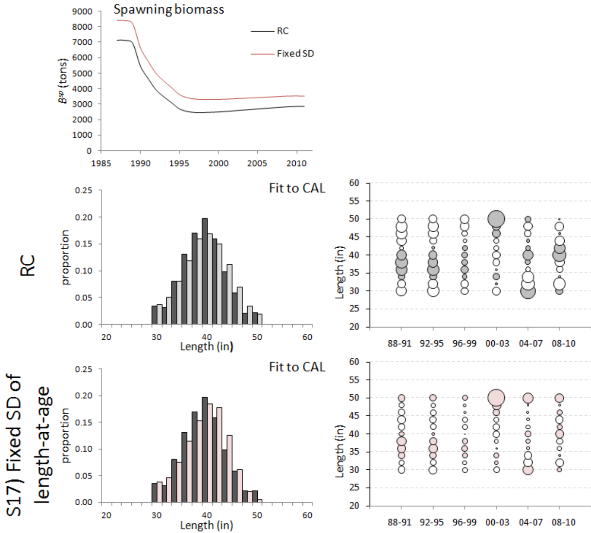
Figure Add.4: Spawning biomass trajectories, and fits to the CAL data (averaged over all the years for which data are available together with bubble plots of residuals) for the RC and the sensitivity fixing the standard deviation of the length-at-age distribution to 78.3 mm based on the Lytton ageing data (S17).
