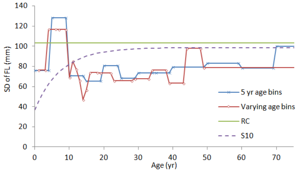
Figure Add.3: Observed standard deviations for the length-at-age distribution for observed ageing data grouped into 5-year age bins and grouped into age bins of varying widths (Lytton, pers. comm) and corresponding estimated values for the RC (constant standard deviation for all ages) and sensitivity S10 in which the standard deviations are assumed proportional to the mean length-at-age.
