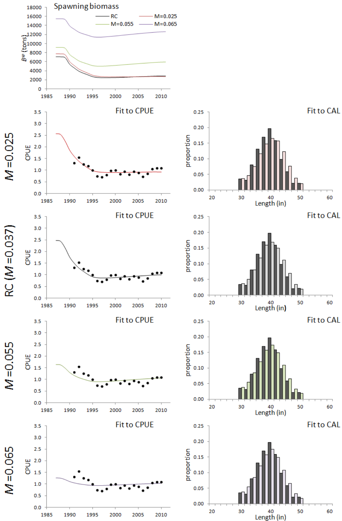
Figure 3: Spawning biomass trajectories showing fits to the CPUE data , together with fits to the CAL data (averaged over all the years for which data are available) for the RC and three sensitivities with different fixed values of natural mortality ( S2a: M=0.025 ; S2b: M=0.055 and S2c: M=0.065 ).
