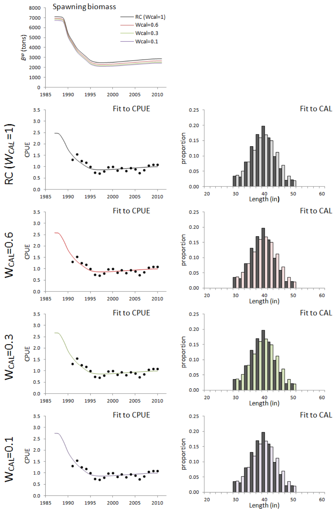
Figure 9: Spawning biomass trajectories, selectivity-at-length and fits to the CPUE and CAL data (averaged over all the years for which data are available) for the RC and three sensitivities with different weighting for the CAL component of -\ln L ( S8 ).
