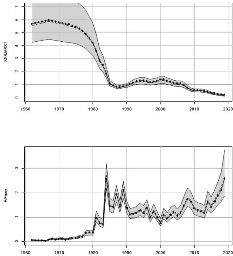
Figure 3.2.1.1. Estimated time series of spawning stock biomass (SSB) and fishing mortality (F) relative to benchmarks. Solid line indicates estimates from base run of the Beaufort Assessment Model; gray error bands indicate 5 th and 95 th percentiles of the ensemble modeling. Top panel: SSB relative to the MSST; if less than 1, stock is overfished. Bottom panel: F relative to F_{MSY} ; if > 1 stock is undergoing overfishing. Source: SEDAR 71 (2021).
