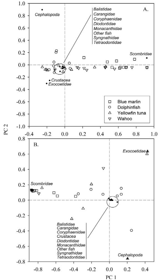
FIGURE 3.—Principal components analysis (%PCA) biplots of annual diet data from four predator species collected during the Big Rock Blue Marlin Tournament (BRT): (A) normalized percent frequency of occurrence (%O; recorded during 10 years: 1998–2000 and 2003–2009) and (B) percent weight (%W; recorded during 7 years: 2003–2009). Open symbols represent predator values. Black circles represent 12 prey taxa used to group diet data. The first and second principal component axes (PC1 and PC2) explained 55.6% and 21.1% of the variation in %O and 59.9% and 19.7% of the variation in %W.
