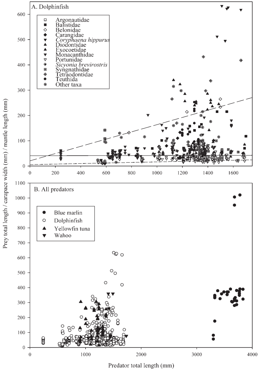
FIGURE 2.—Prey lengths (total length for fishes and shrimps, carapace width for crabs, and mantle length for cephalopods) in predator stomachs versus total length of (A) dolphinfish predators (number of prey measured = 760; Coryphaena hippurus = dolphinfish prey; Sicyonia brevirostris = rock shrimp; lower dashed line = 5th regression quantile, solid line = 50th quantile, upper dashed line = 95th quantile) and (B) all Big Rock Blue Marlin Tournament (BRT)-sampled predators combined (number of prey measured = 854; predators are the blue marlin, dolphinfish, yellowfin tuna, and wahoo). Different symbols represent prey in panel A and predators in panel B. The “other taxa” category in panel A includes the fish taxa Anguilliformes, southern stargazer Astroscopeus y-graecum , manefish Caristius maderensis , conger eel Conger oceanicus , flying gurnard Dactylopterus volitans , round herring Etrumeus teres , Bermuda chub Kyphosus sectatrix , Atlantic tripletail Lobotes surinamensis , Gulf butterflyfish Peprilus burti , Scombridae, and swordfish Xiphias gladius and three invertebrate taxa (Scyllaridae [slipper lobsters], octopus Argonauta nodosa , and sea skater Halobates micans ).
