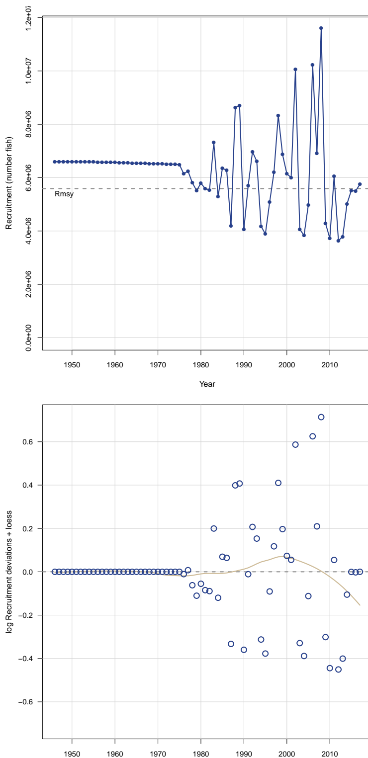
Figure 18. Top panel: Estimated recruitment of age-1 fish. Horizontal dashed line indicates R_{MSY} . Bottom panel: log recruitment residuals. The residual in 2017 was not estimated, as recruitment in that year is uninformed by any data on year-class strength. Thus, the 2017 value shown in the top panel is that predicted from the spawner-recruit curve without deviation.
