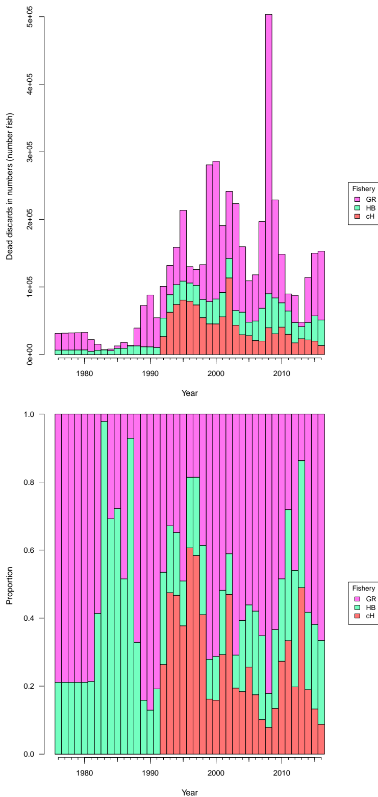
Figure 30. Estimated discard mortalities in numbers by fleet from the catch-age model. cH refers to commercial handlines, HB to headboat, and GR to general recreational.
