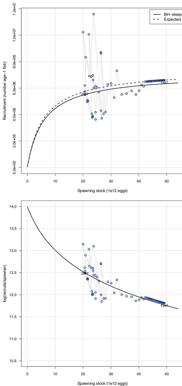
Figure 32. Top panel: Beverton–Holt spawner-recruit curves, with and without lognormal bias correction. The expected (upper) curve was used for computing management benchmarks. Bottom panel: log of recruits (number age-1 fish) per spawner as a function of spawners.
