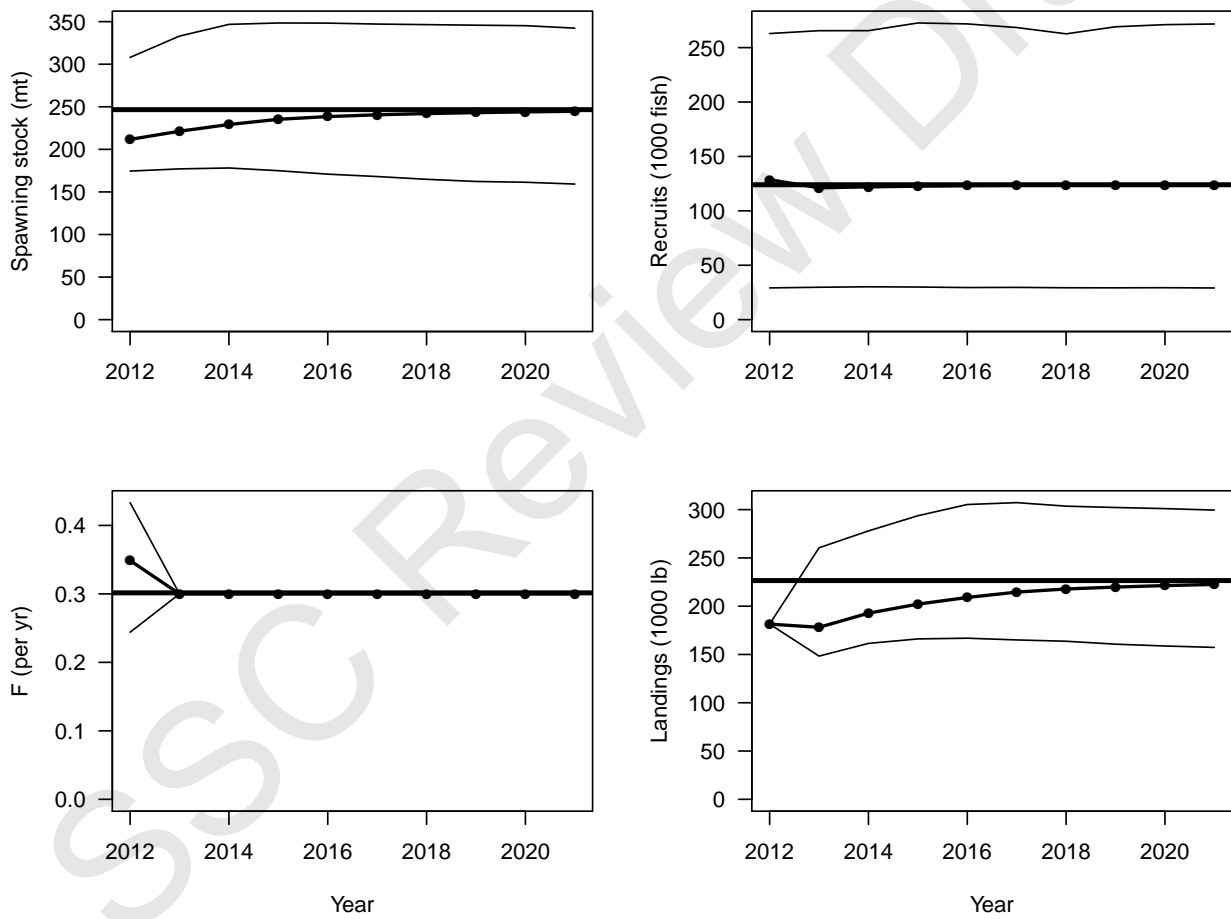
Figure 3.49. Projection results under scenario 2—fishing mortality rate fixed at F = F_{\text{rebuild}} = 0.30 . Expected values represented by dotted solid lines, and uncertainty represented by thin lines corresponding to 5 th and 95 th percentiles of replicate projections. Horizontal lines mark MSY-related quantities. Spawning stock (SSB) is at time of peak spawning.
