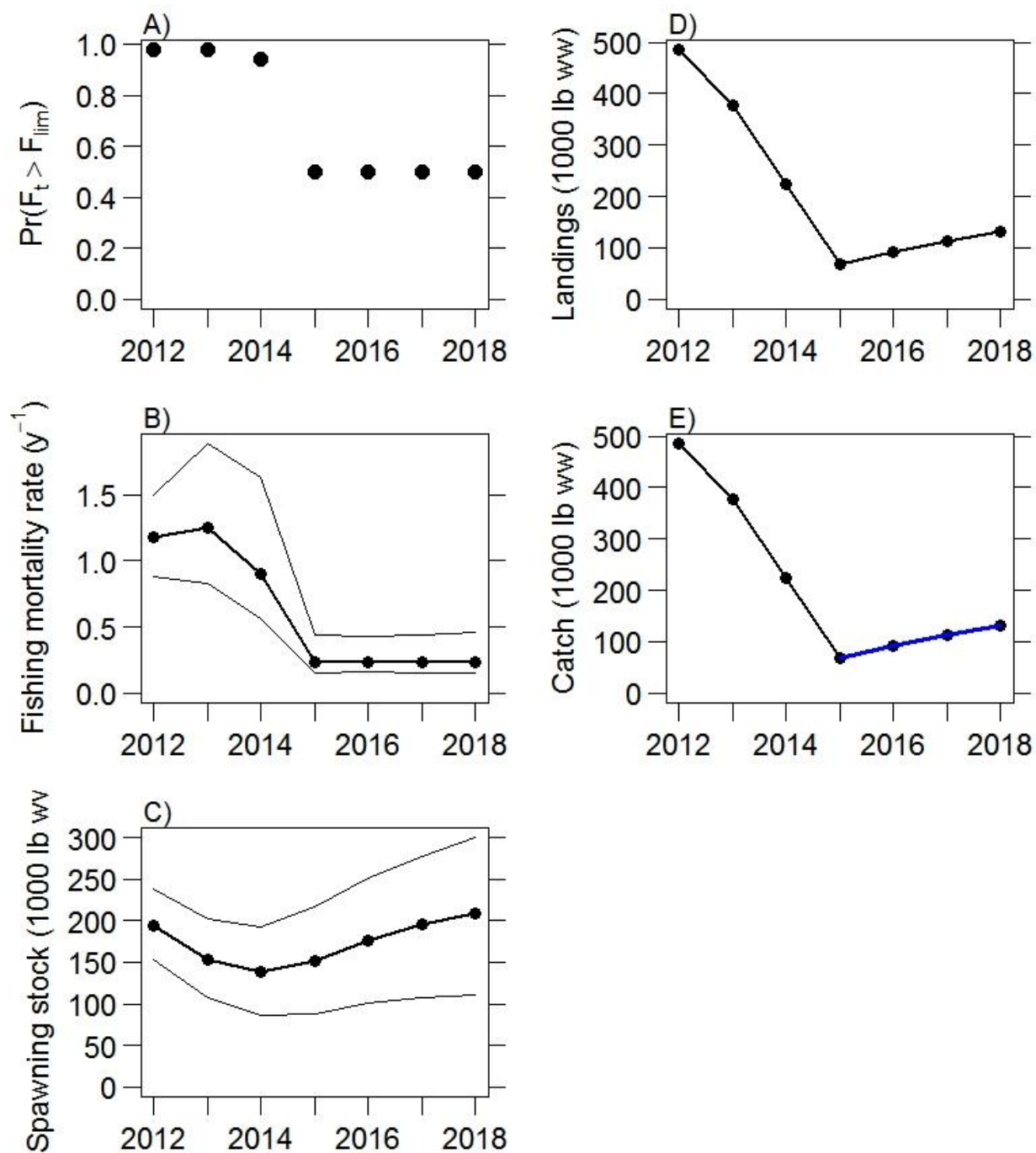
Figure 2. P^* = 0.5 projection results. For this assessment, discards were combined with landings so the ABC reflects both landings and dead discards (i.e., landings = catch). Annual ABCs (panel E) are a single quantity while other values presented are medians. Error bars represent the 5 th and 95 th percentiles of the 10,000 projection runs.
