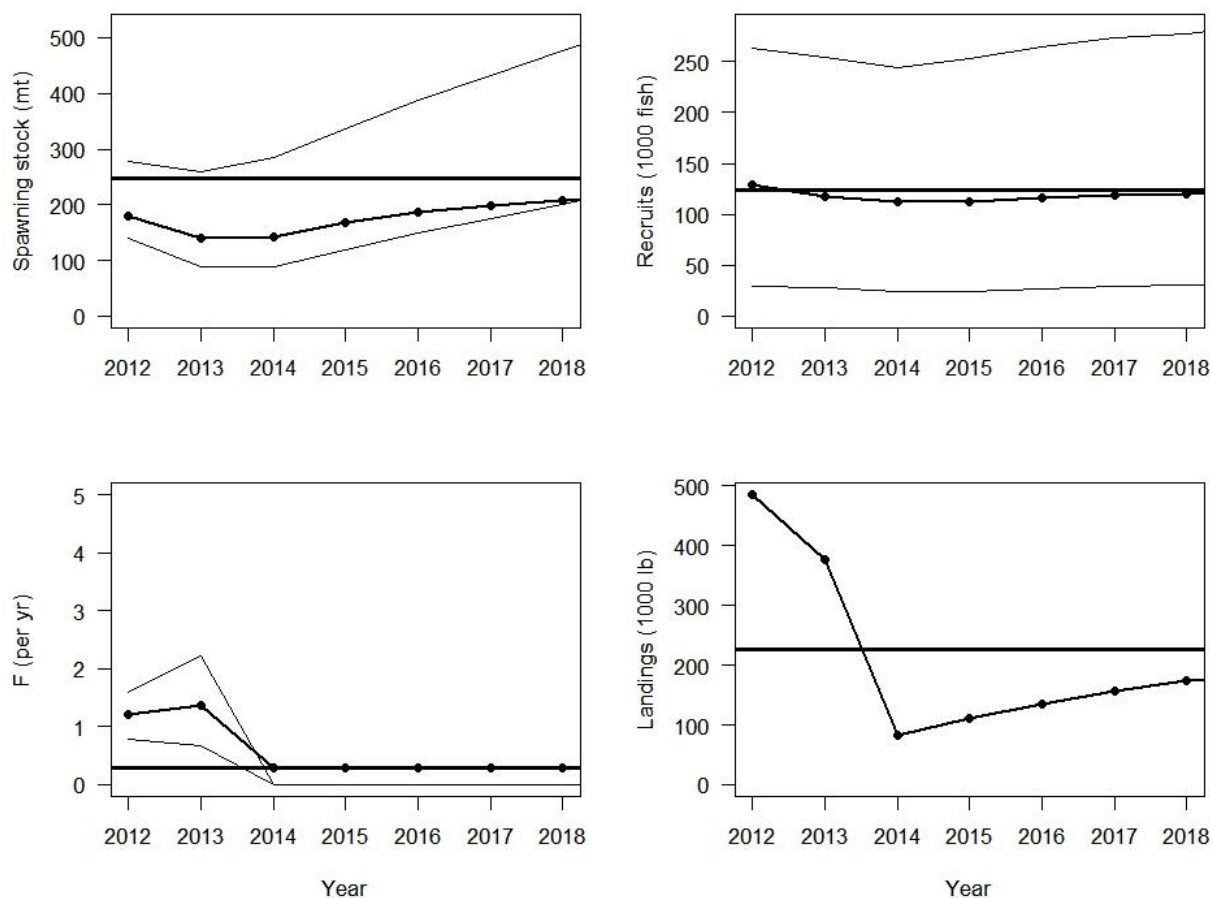
Figure 5. Scenario 3: Constant F projection at F=F_{msy} . For this assessment, discards were combined with landings so the ABC reflects both landings and dead discards (landings and dead discards are separated in the associated Tables. Annual ABCs (panel E) are a single quantity while other values presented are medians. Error bars represent the 5 th and 95 th percentiles of the 10,000 projection runs.
