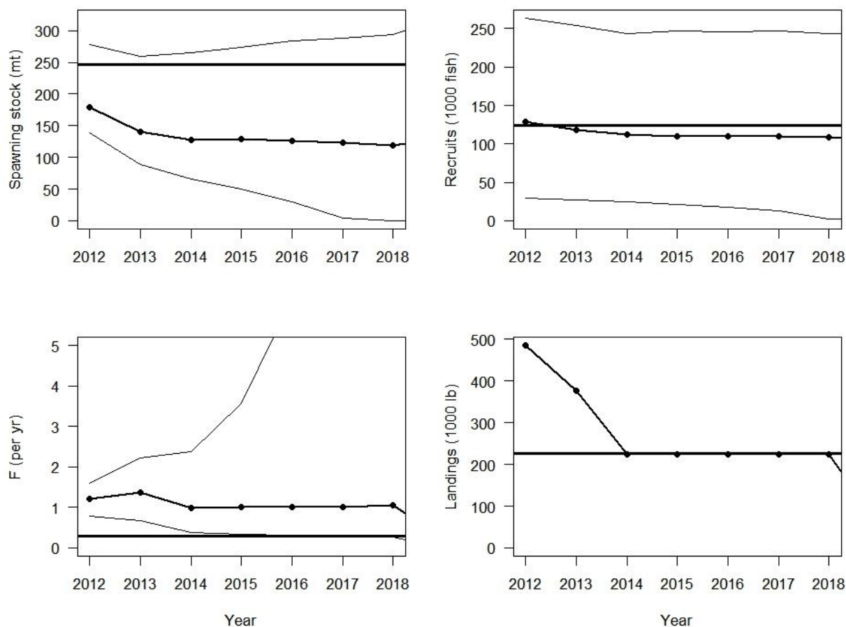
Figure 3. Scenario 1: Landings set to the yield that would result at F=75\%F_{msy} under equilibrium conditions (224.1 klb). For this assessment, discards were combined with landings so the ABC reflects both landings and dead discards (landings and dead discards are separated in the associated Tables). Error bars represent the 5 th and 95 th percentiles of the 10,000 projection runs.
