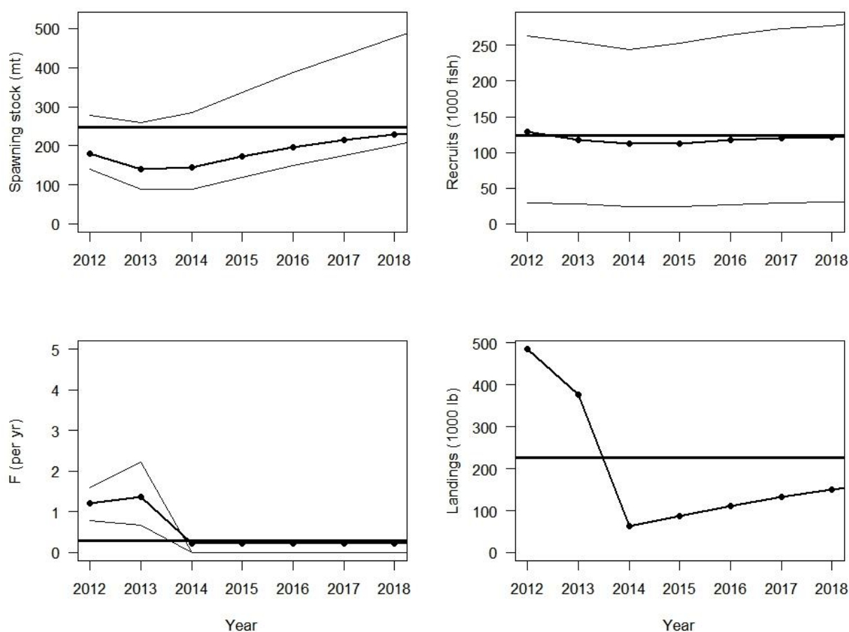
Figure 4. Scenario 2: Constant F projection at F=75\%F_{msy} . For this assessment, discards were combined with landings so the ABC reflects both landings and dead discards (landings and dead discards are separated in the associated Tables. Annual ABCs (panel E) are a single quantity while other values presented are medians. Error bars represent the 5 th and 95 th percentiles of the 10,000 projection runs.
