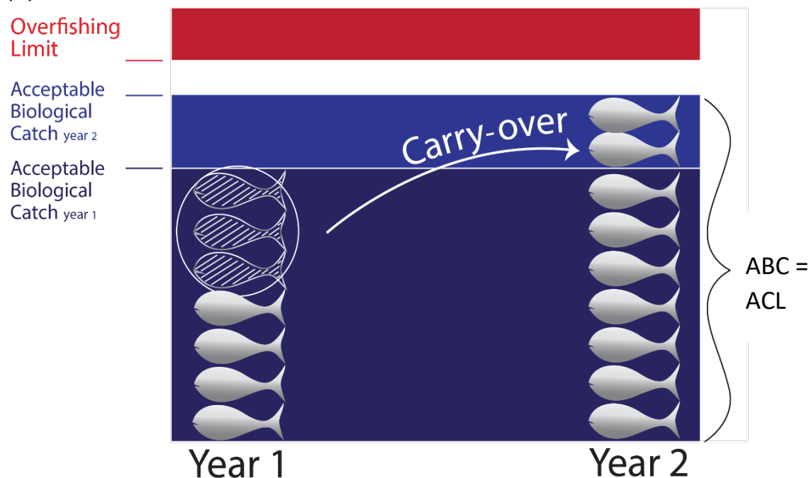
Figure 1. Examples of carry-over approaches: (a) utilizes the buffer between ACL and ABC, and (b) adjusts the ABC. In (a), actual catches in year 1 were less than the ACL. A portion of the catch underage was carried-over to increase the ACL in year 2, which is less than the ABC. In (b) the ACL and ABC are set equal to each other, and actual catches in year 1 were less than the ACL. A portion of the catch underage was carried-over to increase the ABC in year 2. The NS1 guidelines allow ABC control rules to include provisions for the carry-over of some of the unused portion of the ACL from one year to increase the ABC for the next year.
