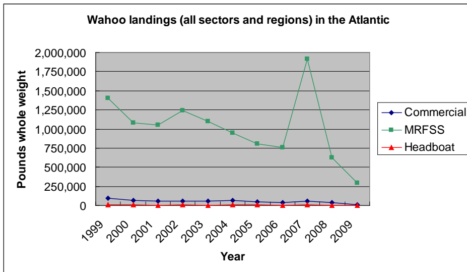
Figure 4. Annual commercial, MRFSS, and headboat landings (lbs whole weight) of wahoo in the Atlantic, 1999 – 2009. Data are inclusive of all the states within the jurisdiction of the New England, Mid-Atlantic, and South Atlantic Fishery Management Councils. Data are not reported by state due to confidentiality concerns. Data for 2009 are incomplete. Headboat data are from the South Atlantic region.
