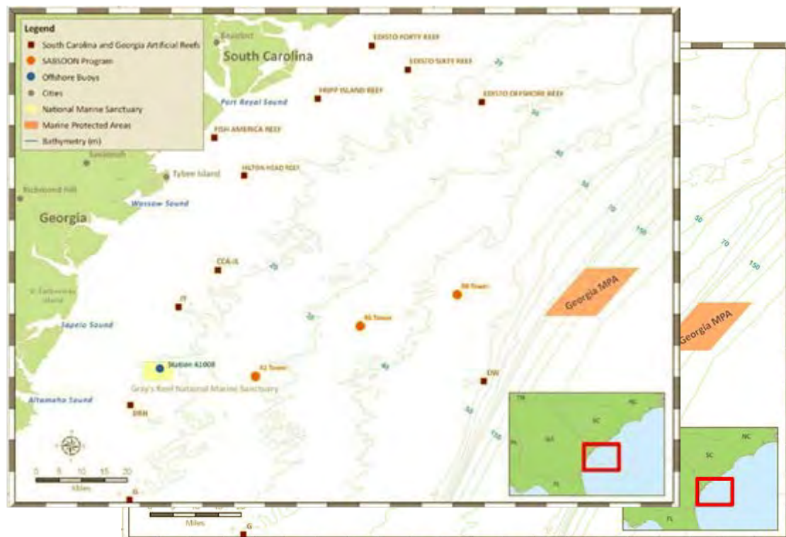
Figure 8. The Georgia MPA, located east of Wassaw Sound, GA (SAFMC 2009).
