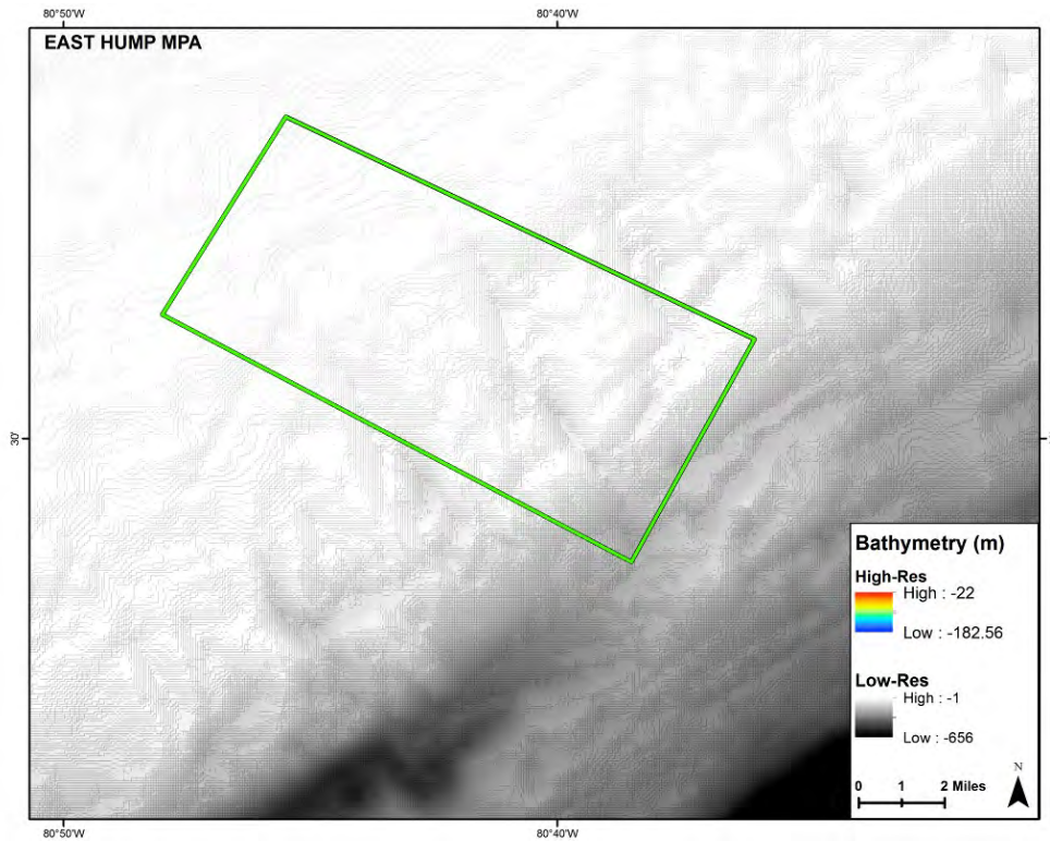
Figure 16. Low-resolution bathymetry of the East Hump MPA (Provided by N. Farmer).
