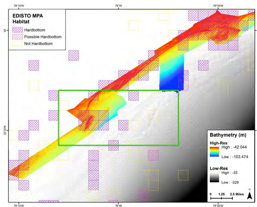
Figure 6. Low- and high-resolution bathymetry and habitat characterization within and outside of the Edisto MPA (Provided by N. Farmer).
