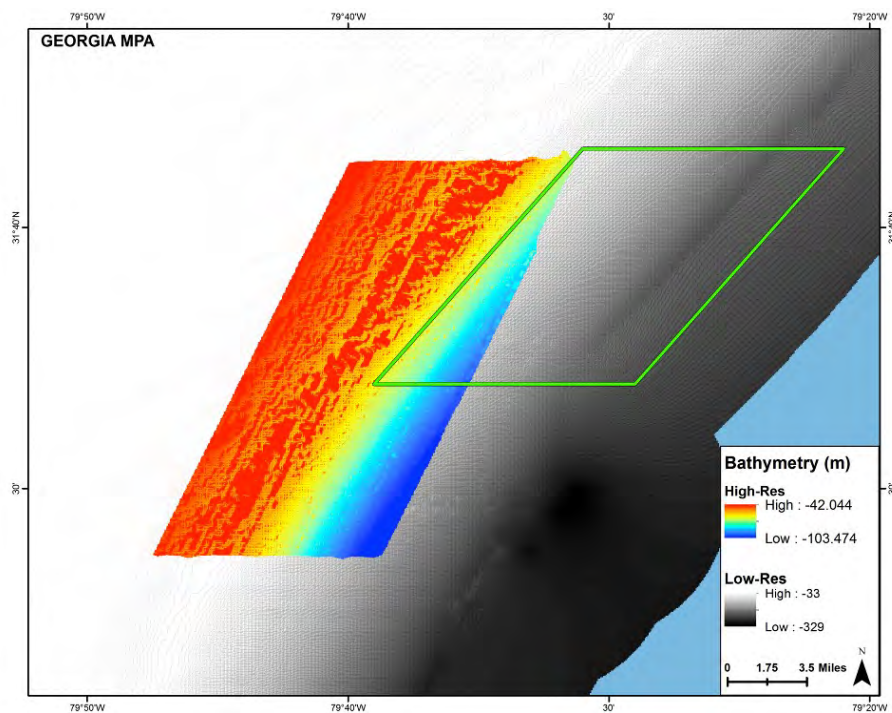
Figure 9. Low- and high-resolution bathymetry within and outside of the Georgia MPA (Provided by N. Farmer).
