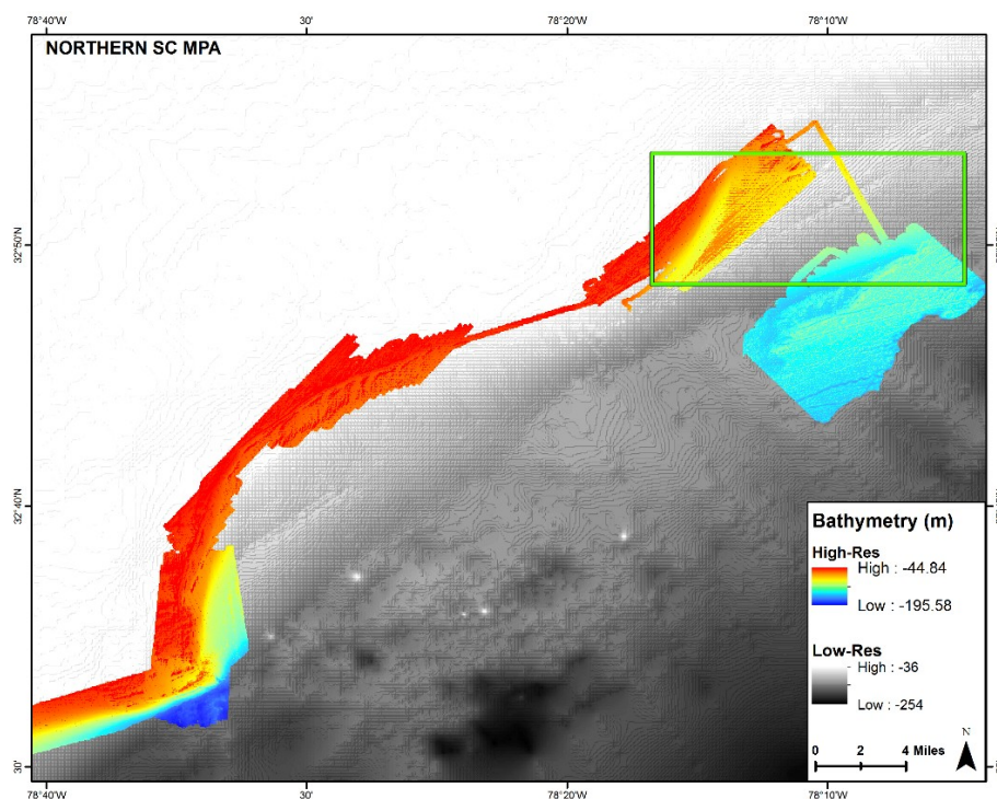
Figure 4.2.2. Low- and high-resolution bathymetry within and outside of the Northern South Carolina MPA (Provided by N. Farmer).
