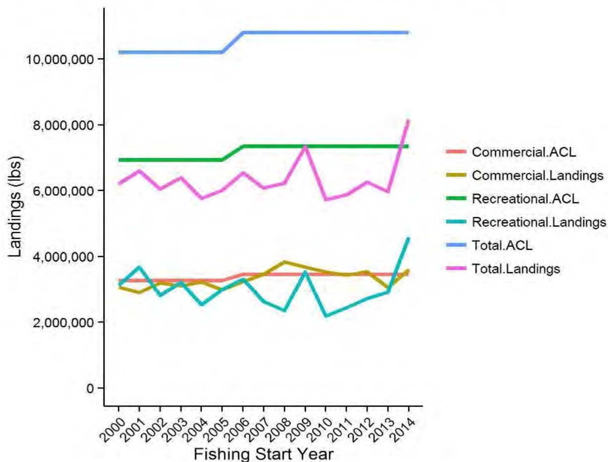
Figure 2.8.1. Trends in Gulf king mackerel landings by sector for the 2000-01 to the 2014-15 fishing seasons. Landings are in pounds.
