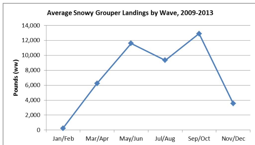
Figure 3.3.1.57. Average snowy grouper landings (lb ww) by wave, 2009–2013. Source: SEFSC ACL Recreational Dataset (mrfsassess_rec81_13wv6_24feb14).
