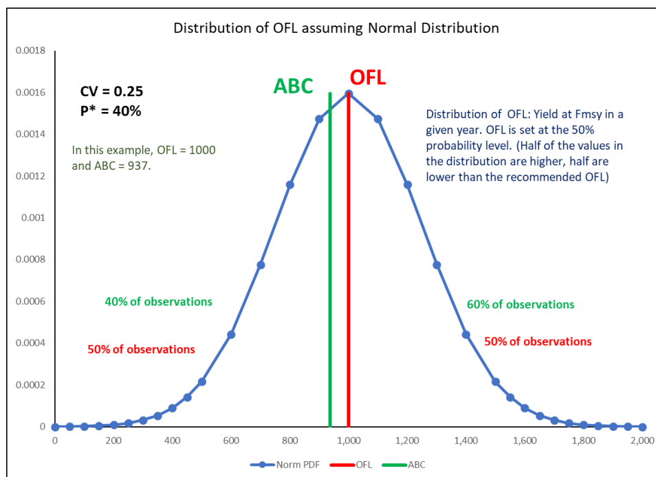
Figure App H.2. Example distribution illustrating OFL and ABC for a hypothetical stock with OFL=1000 pounds, a chosen risk tolerance or P^* of 40% (40% chance that overfishing occurs), and an assessment CV of 0.25.
