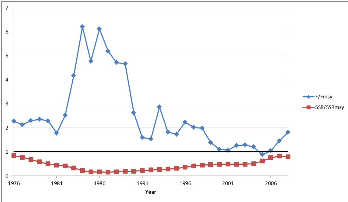
Figure 4. Spawning stock biomass (SSB) and exploitation (F) levels relative to expected conditions of the red grouper stock at MSY. Relative biomass is depicted by SSB/SSB MSY and exploitation by F/F MSY . The index line at 1 represents MSY conditions. Data are from the SEDAR 19 report for red grouper.
