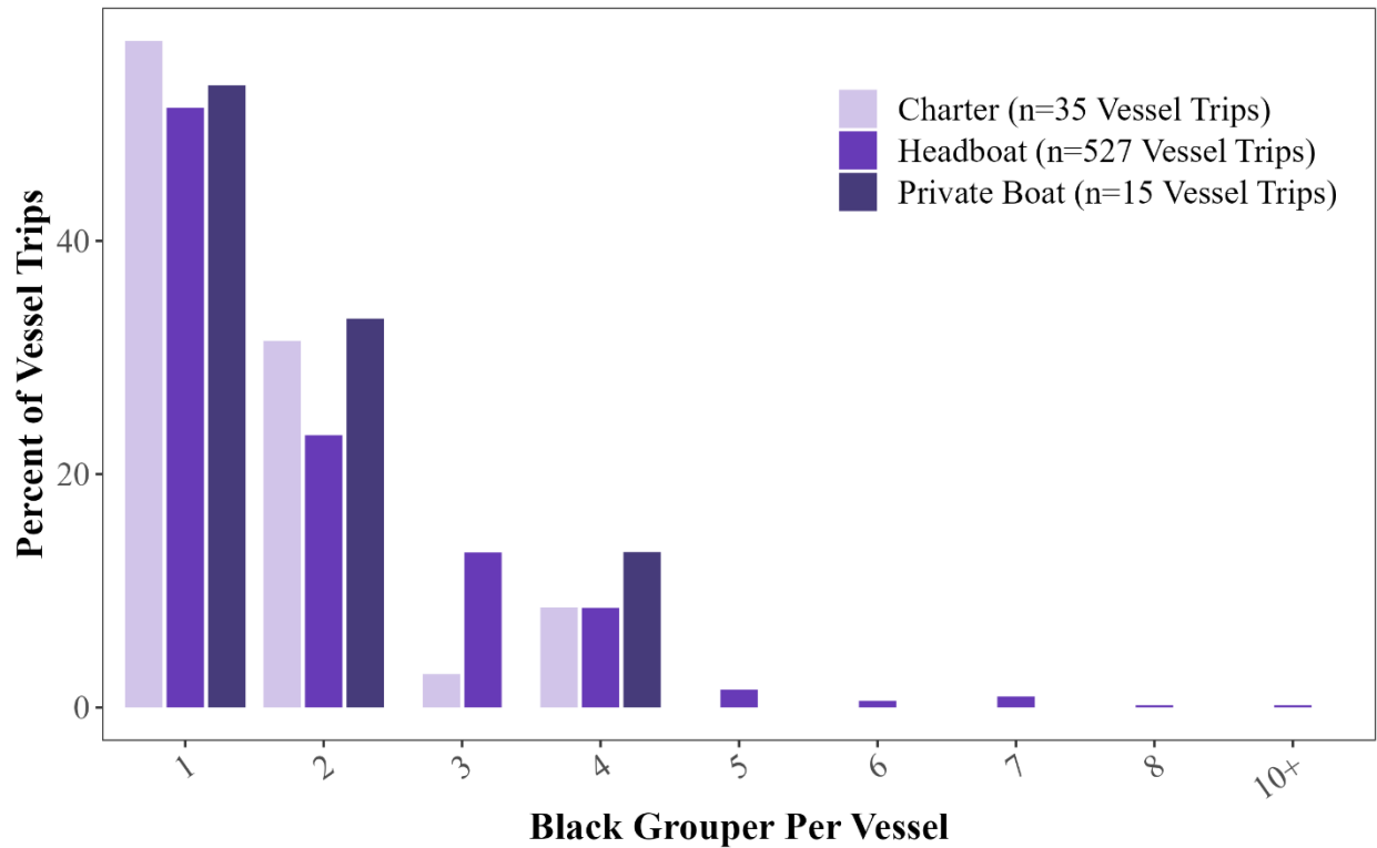
Figure E.4. Distribution of black grouper vessel harvest from dockside intercept and headboat logbook data from 2018-2022, by recreational fleet.
