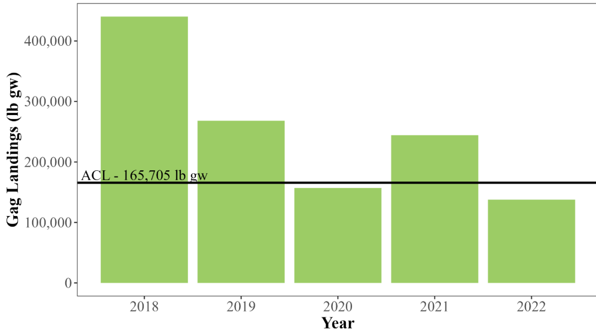
Figure E.1. Annual gag landings from 2018 through 2022 in pounds whole weight, using MRFSS units. The current recreational ACL is represented by a solid horizontal black line. Data Source: SEFSC MRFSS ACL Monitoring – Feb 2024.
