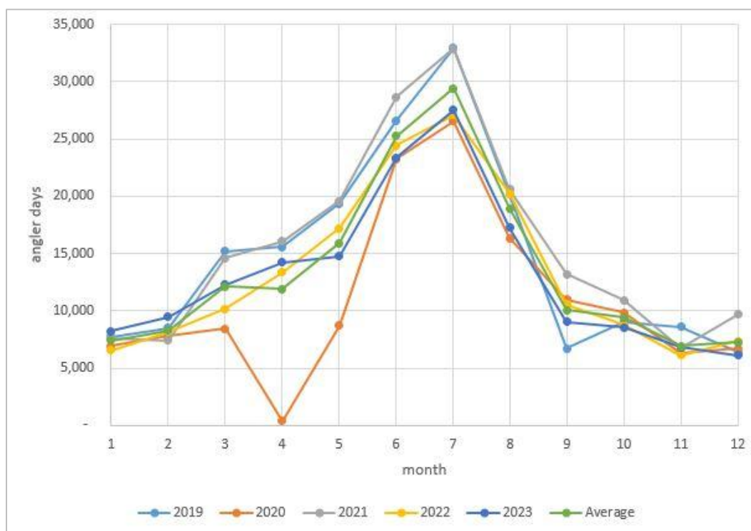
Figure 3.3.2.3. South Atlantic headboat angler days by month and year (2019-2023).
