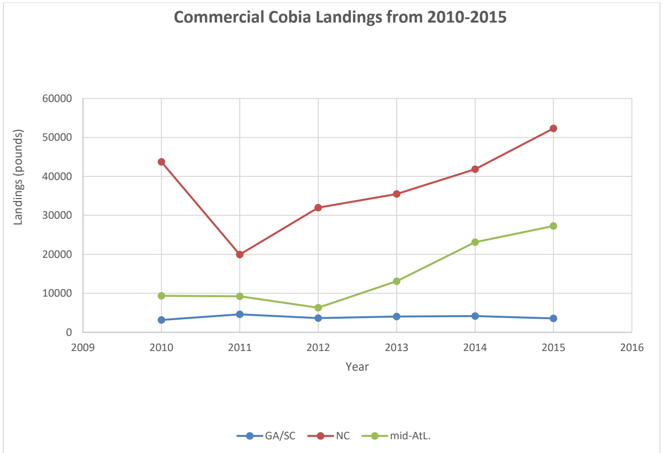
Figure 4. Commercial landings of Cobia (2010-2015)
