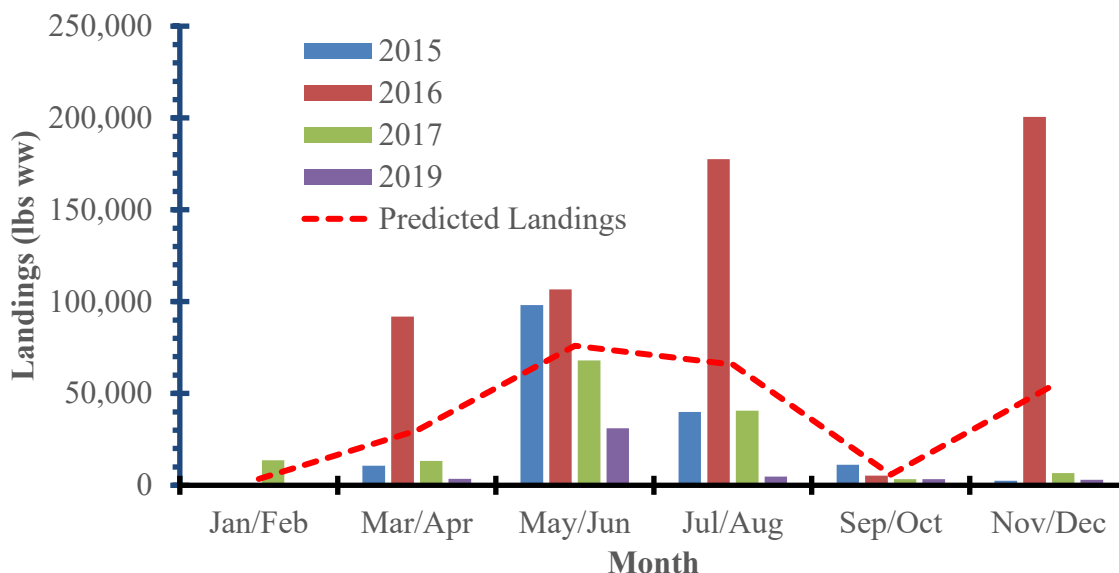
Figure 4.5.2.1. South Atlantic red porgy recreational landings by two-month wave and predicted future landings.
